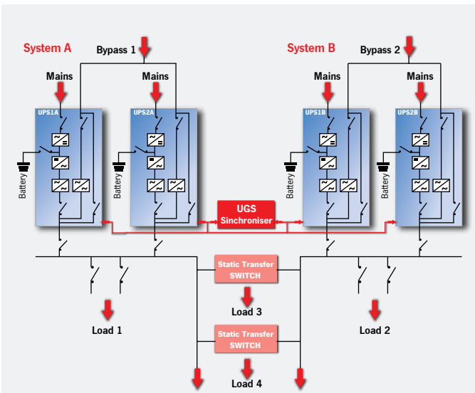
Dynamic dual bus configuration Solution that ensures redundancy until the distribution of the powersupply to the loads + Downstream fault discrimination
